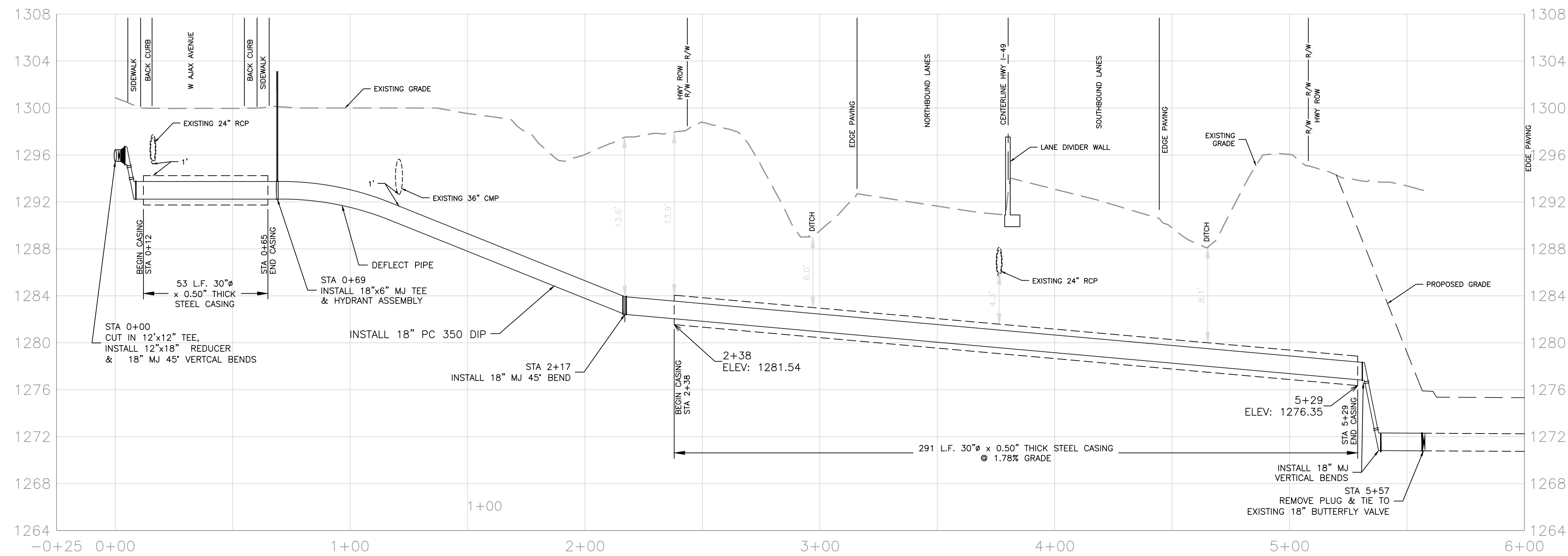
PROFILE WATER LINE 1 STA 0+00 TO 5+57 SCALE: HORIZ 1"=30' / VERT 1"= 6'
